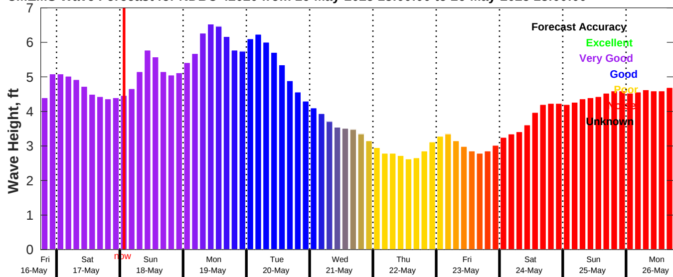
CMEMS Wave Forecast for NDBC 42020 from 16-May-2025 18:00:00 to 26-May-2025 18:00:00
