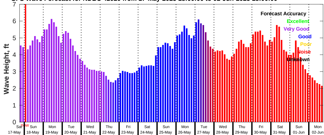
GFS Wave Forecast for NDBC 42020 from 17-May-2025 18:00:00 to 02-Jun-2025 18:00:00
