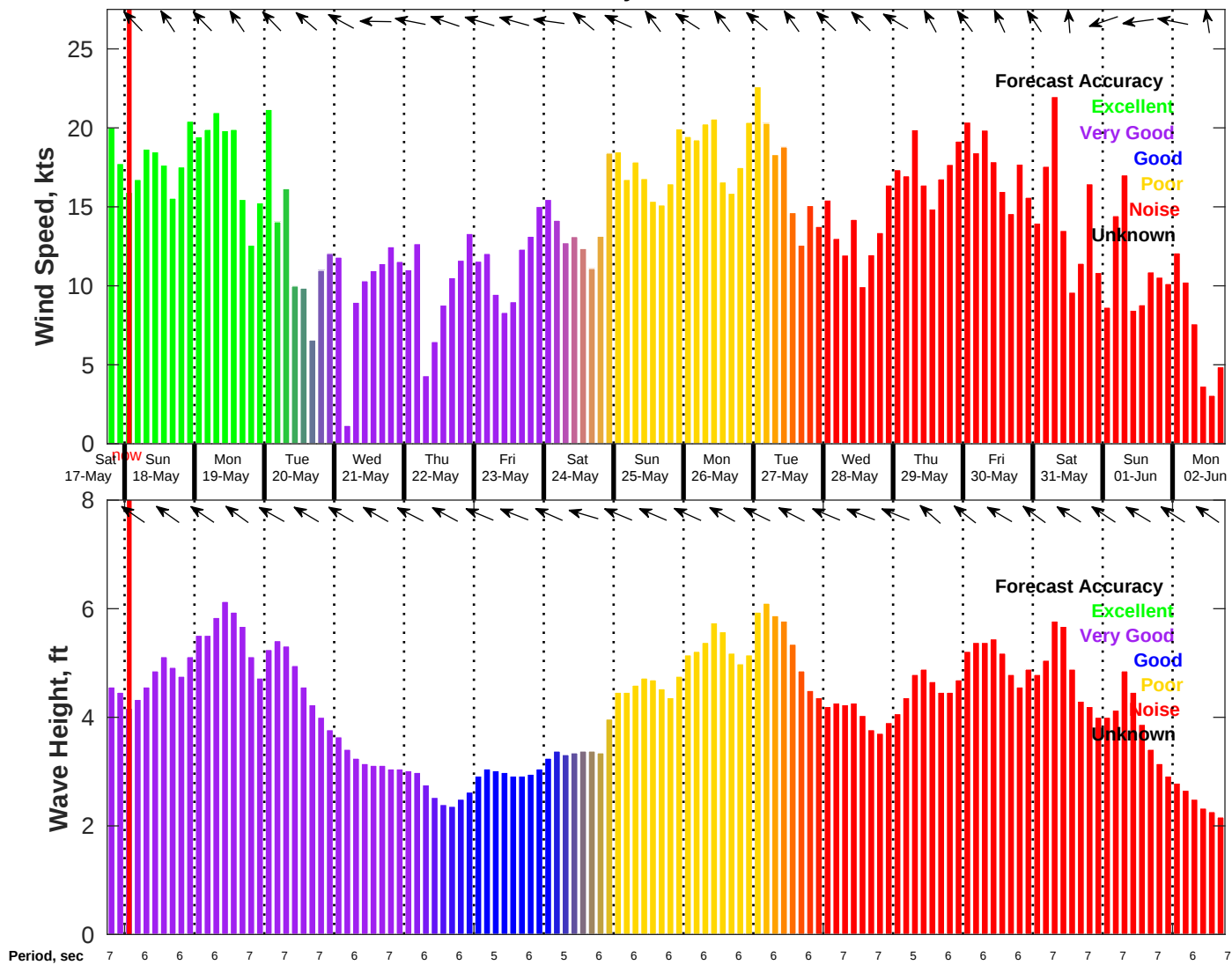
Wind & Wave Forecast for NDBC 42020 from 17-May-2025 18:00:00 to 02-Jun-2025 18:00:00
