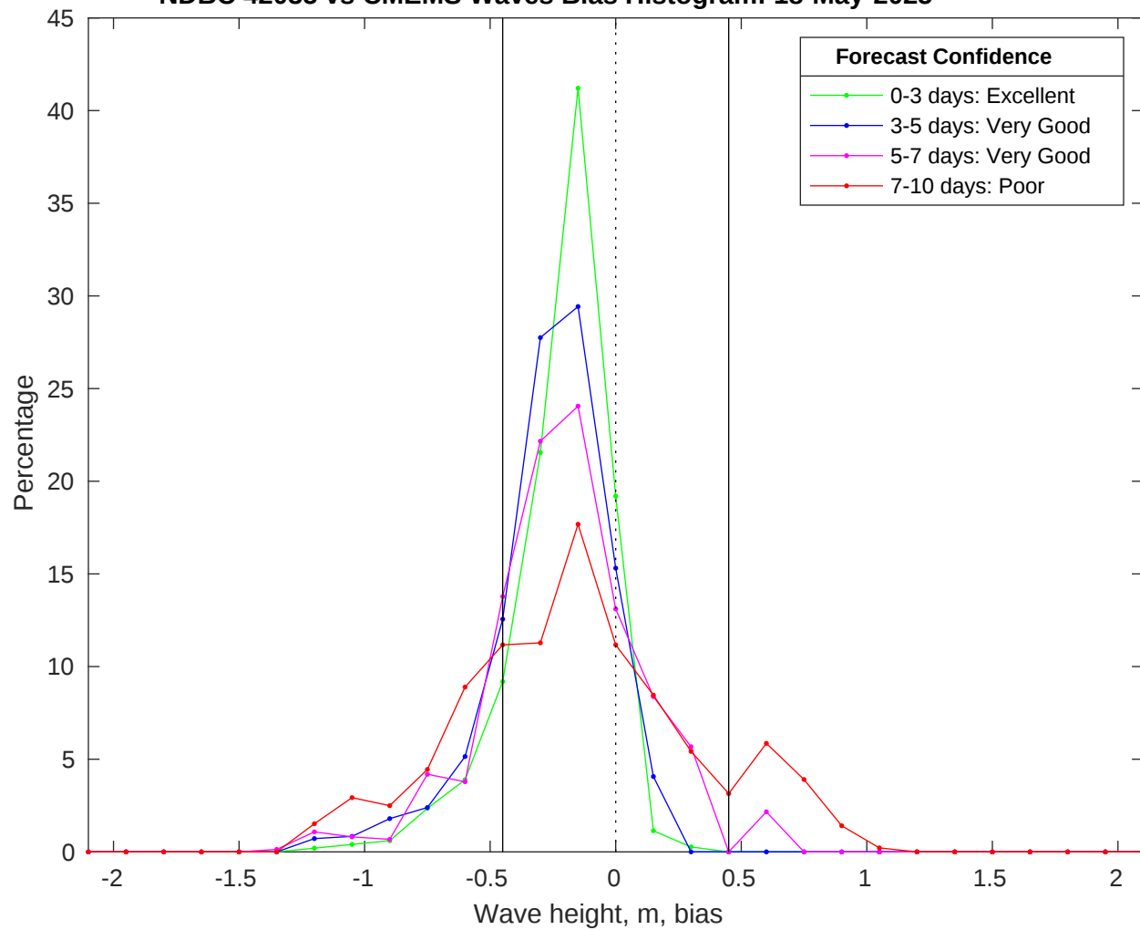
NDBC 42035 vs CMEMS Waves Bias Histogram: 18-May-2025
