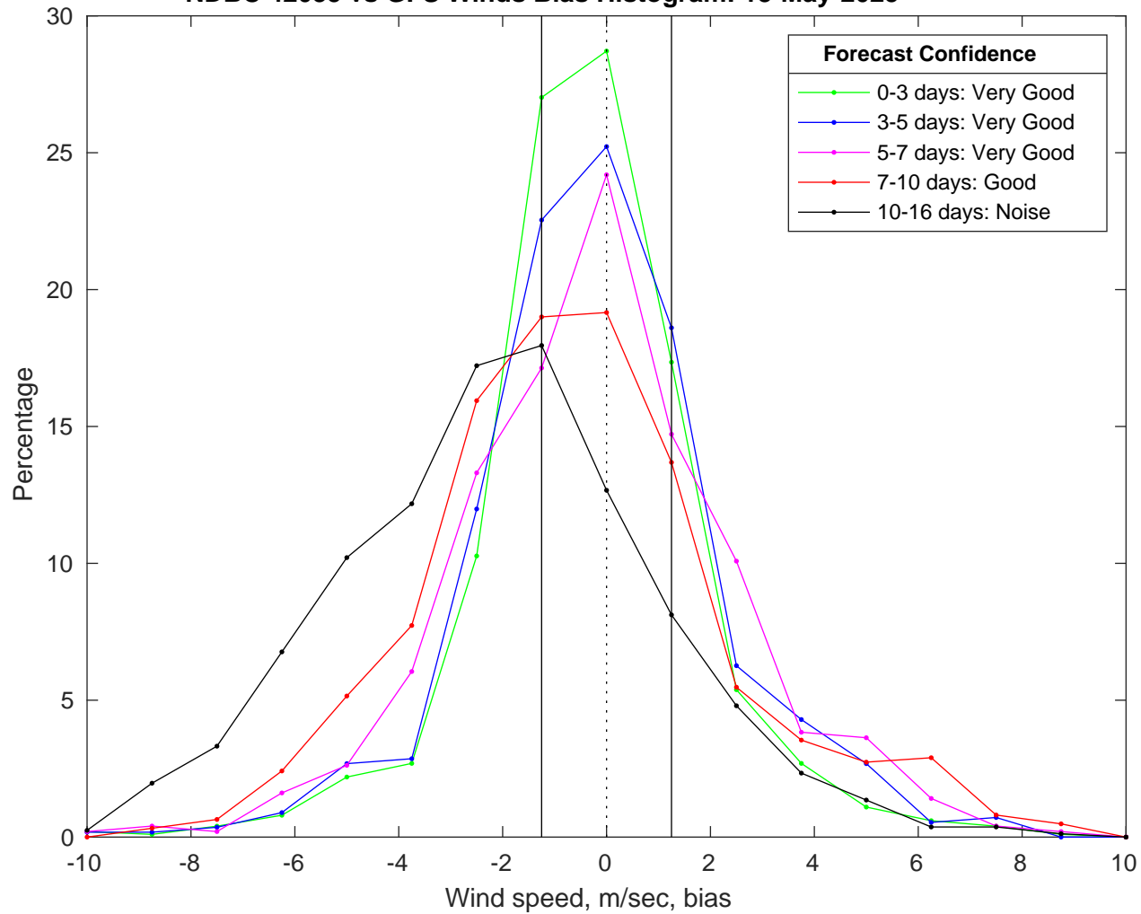
NDBC 42035 vs GFS Winds Bias Histogram: 18-May-2025
