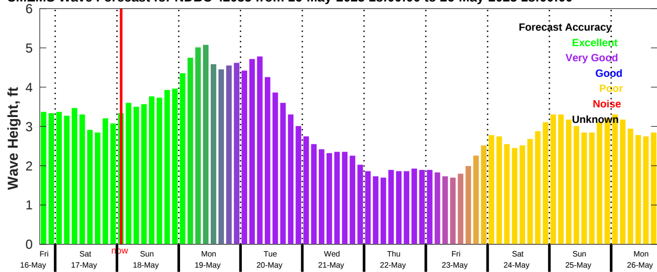
CMEMS Wave Forecast for NDBC 42035 from 16-May-2025 18:00:00 to 26-May-2025 18:00:00
