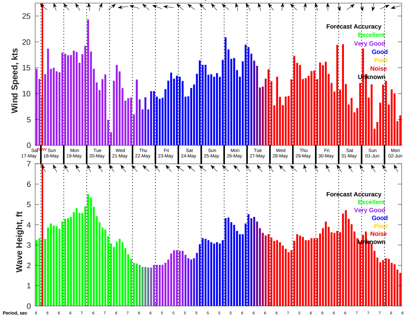
Wind & Wave Forecast for NDBC 42035 from 17-May-2025 18:00:00 to 02-Jun-2025 18:00:00
