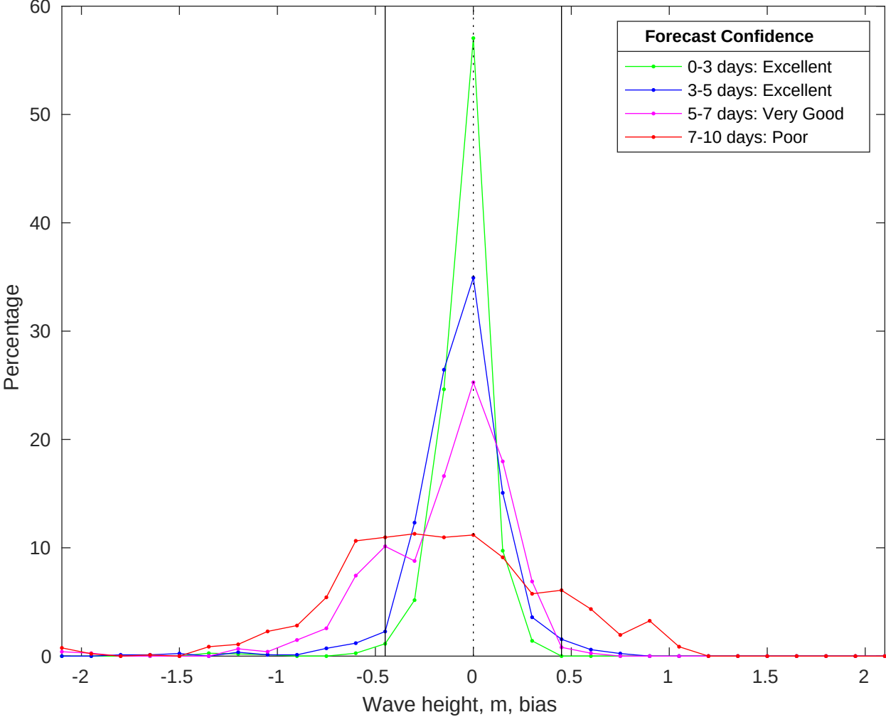
NDBC 42036 vs CMEMS Waves Bias Histogram: 18-May-2025
