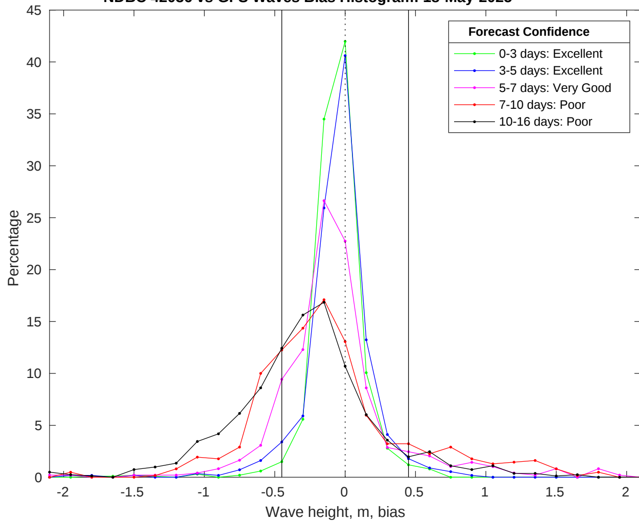
NDBC 42036 vs GFS Waves Bias Histogram: 18-May-2025
