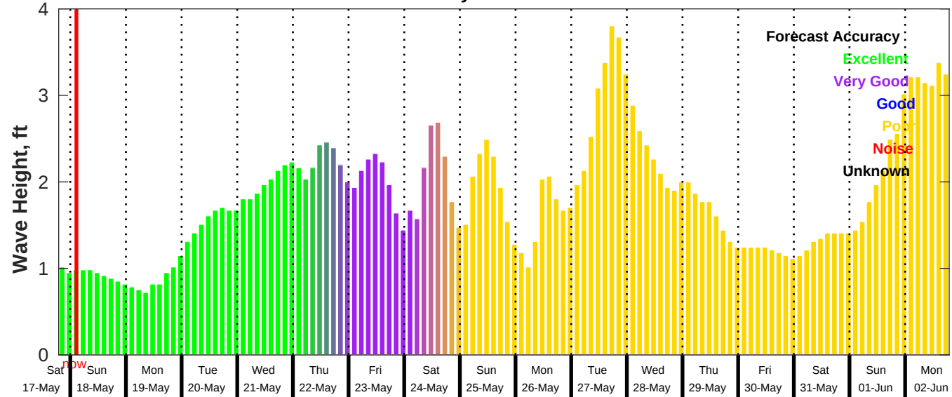
GFS Wave Forecast for NDBC 42036 from 17-May-2025 19:00:00 to 02-Jun-2025 19:00:00
