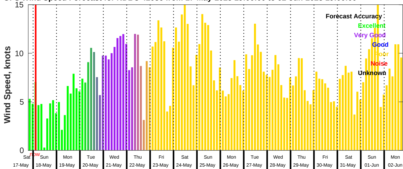
GFS Wind Speed Forecast for NDBC 42036 from 17-May-2025 19:00:00 to 02-Jun-2025 19:00:00
