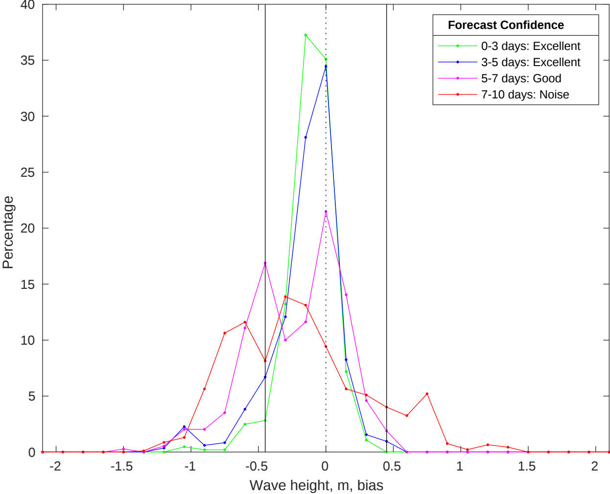
NDBC 42040 vs CMEMS Waves Bias Histogram: 18-May-2025
