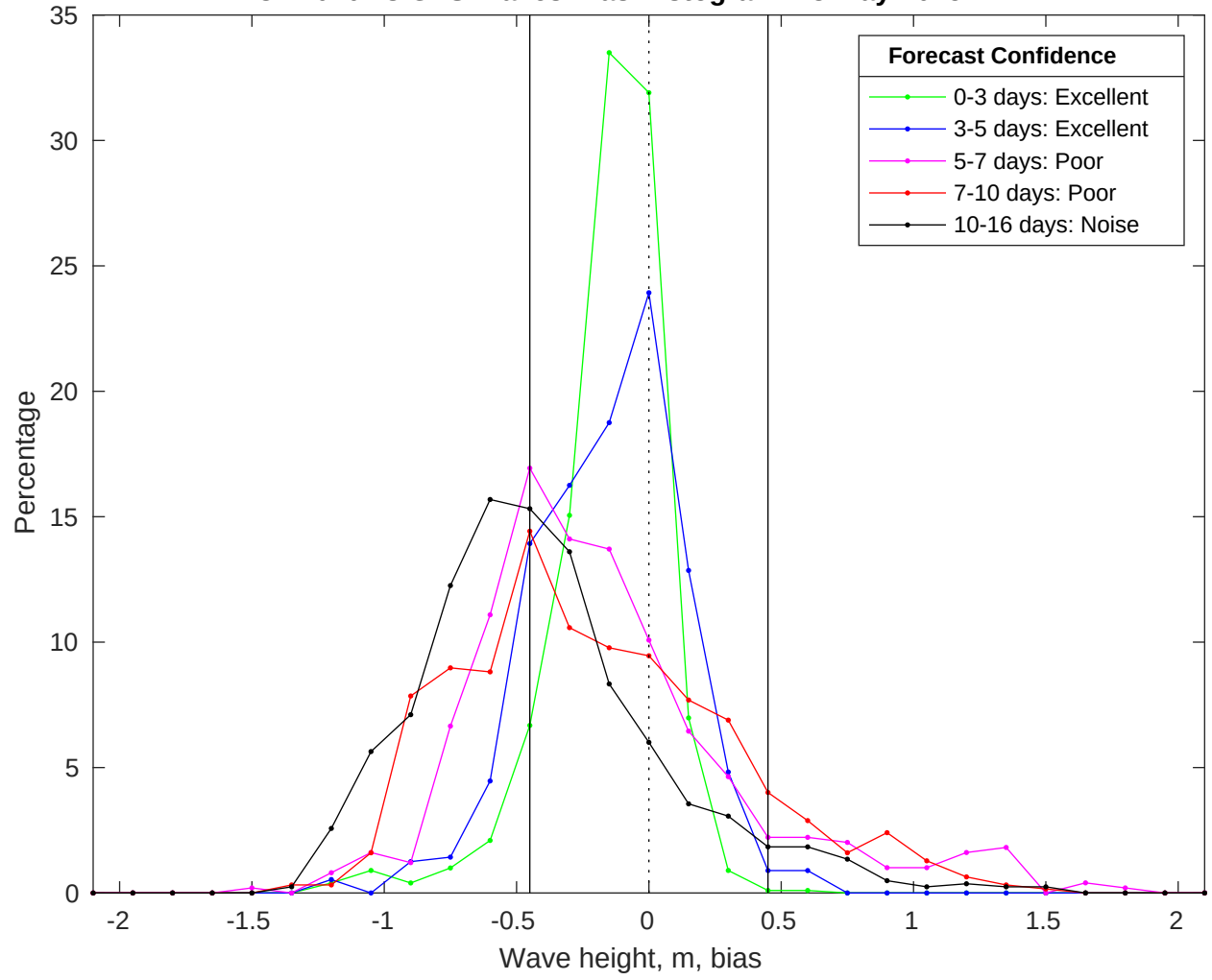
NDBC 42040 vs GFS Waves Bias Histogram: 18-May-2025
