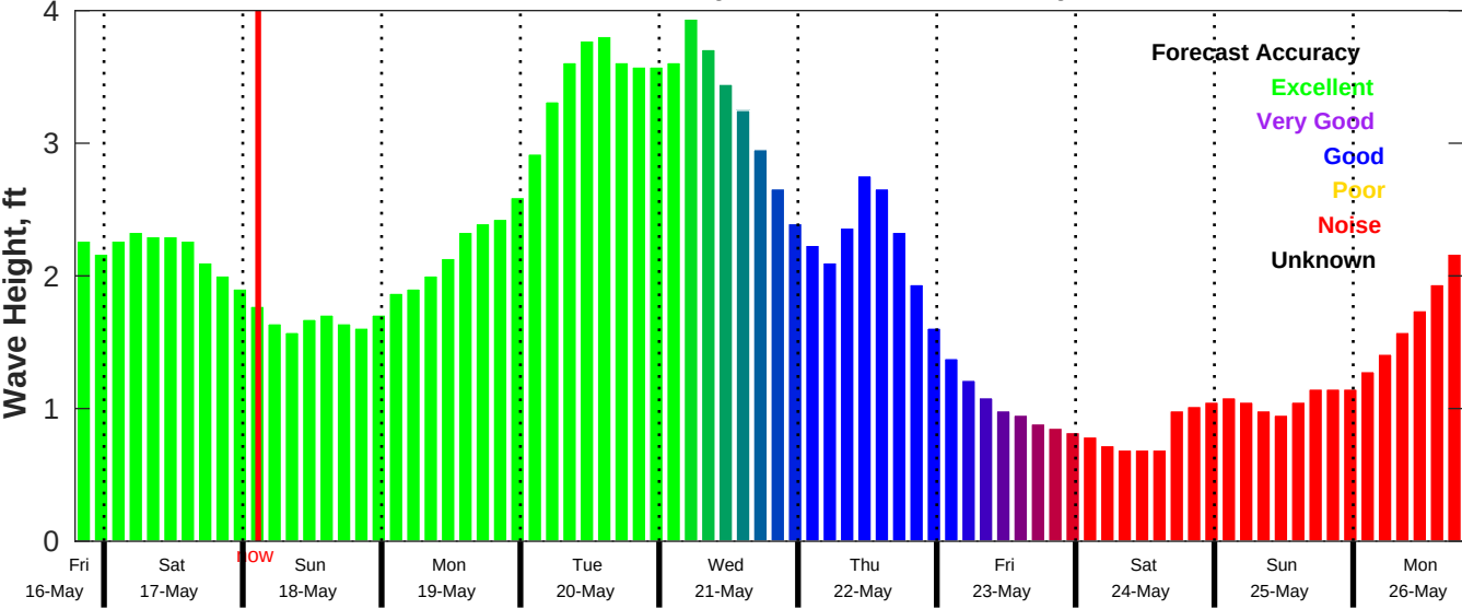
CMEMS Wave Forecast for NDBC 42040 from 16-May-2025 19:00:00 to 26-May-2025 19:00:00
