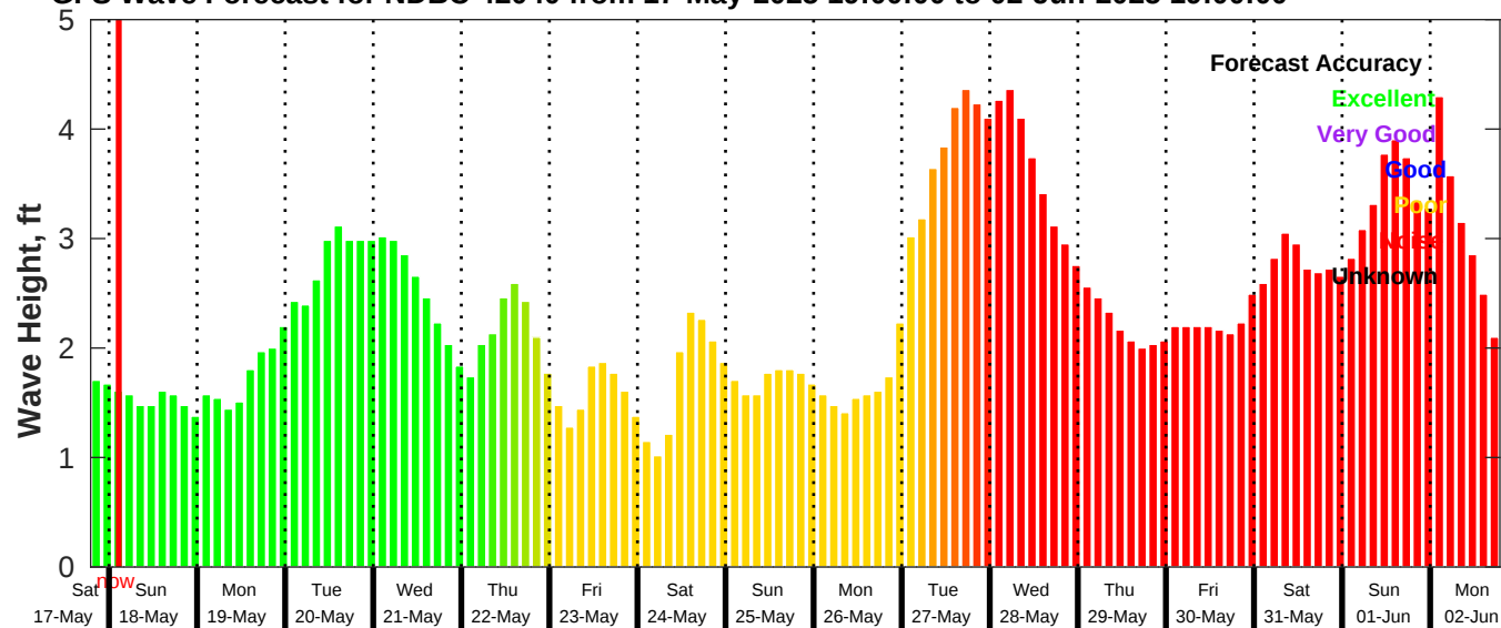
GFS Wave Forecast for NDBC 42040 from 17-May-2025 19:00:00 to 02-Jun-2025 19:00:00
