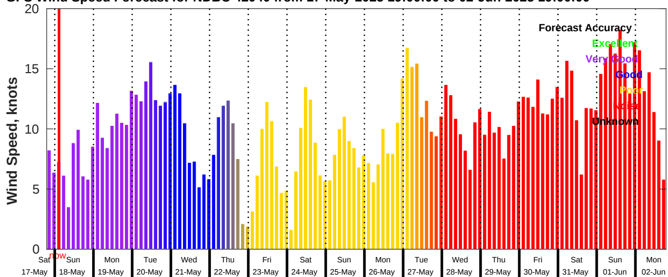
GFS Wind Speed Forecast for NDBC 42040 from 17-May-2025 19:00:00 to 02-Jun-2025 19:00:00
