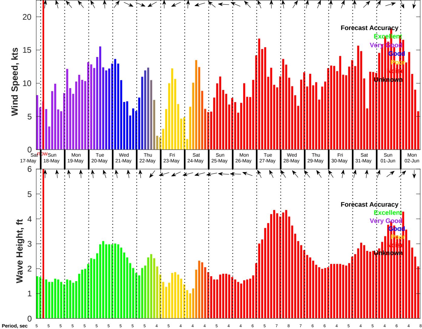
Wind & Wave Forecast for NDBC 42040 from 17-May-2025 19:00:00 to 02-Jun-2025 19:00:00
