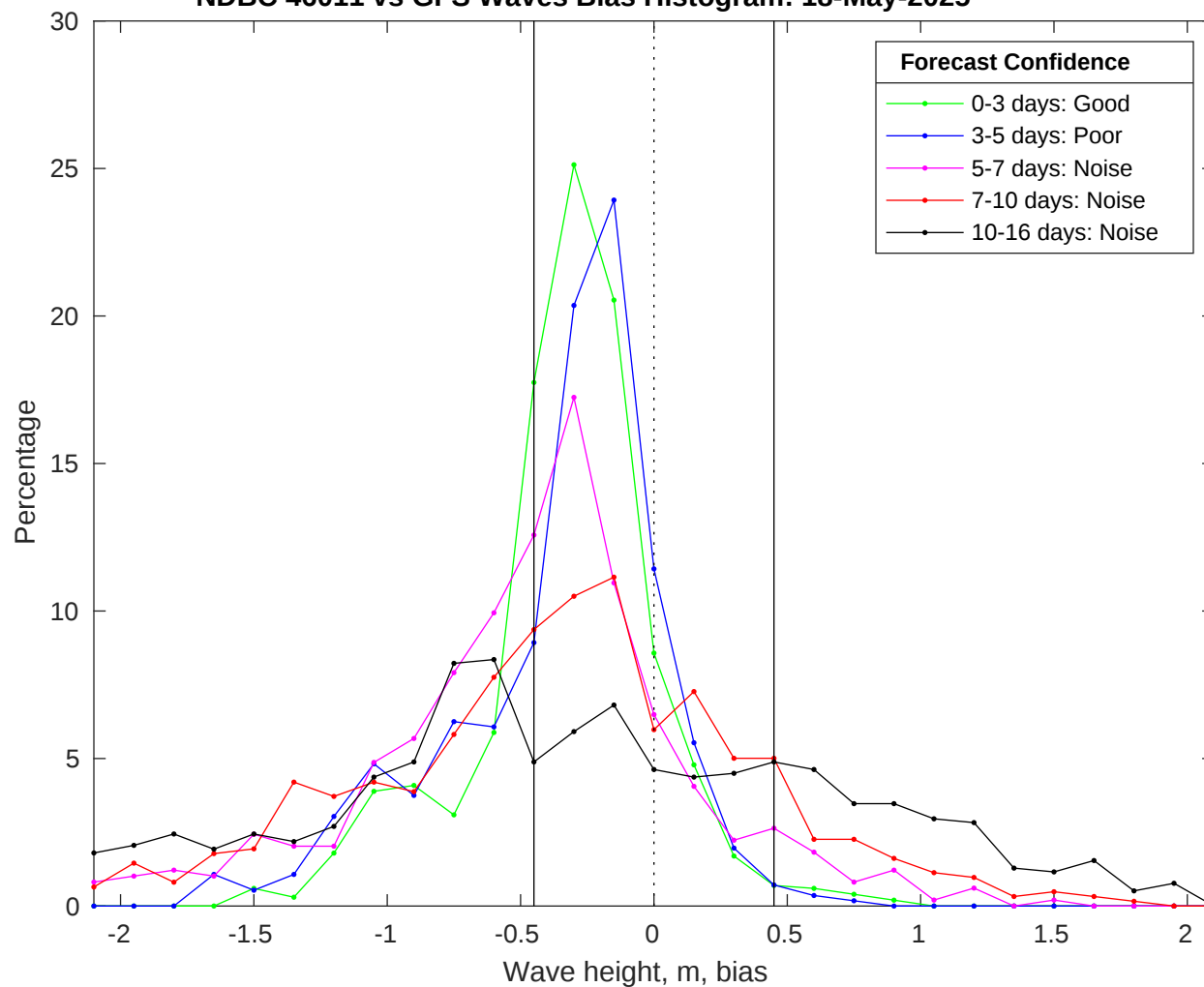
NDBC 46011 vs GFS Waves Bias Histogram: 18-May-2025
