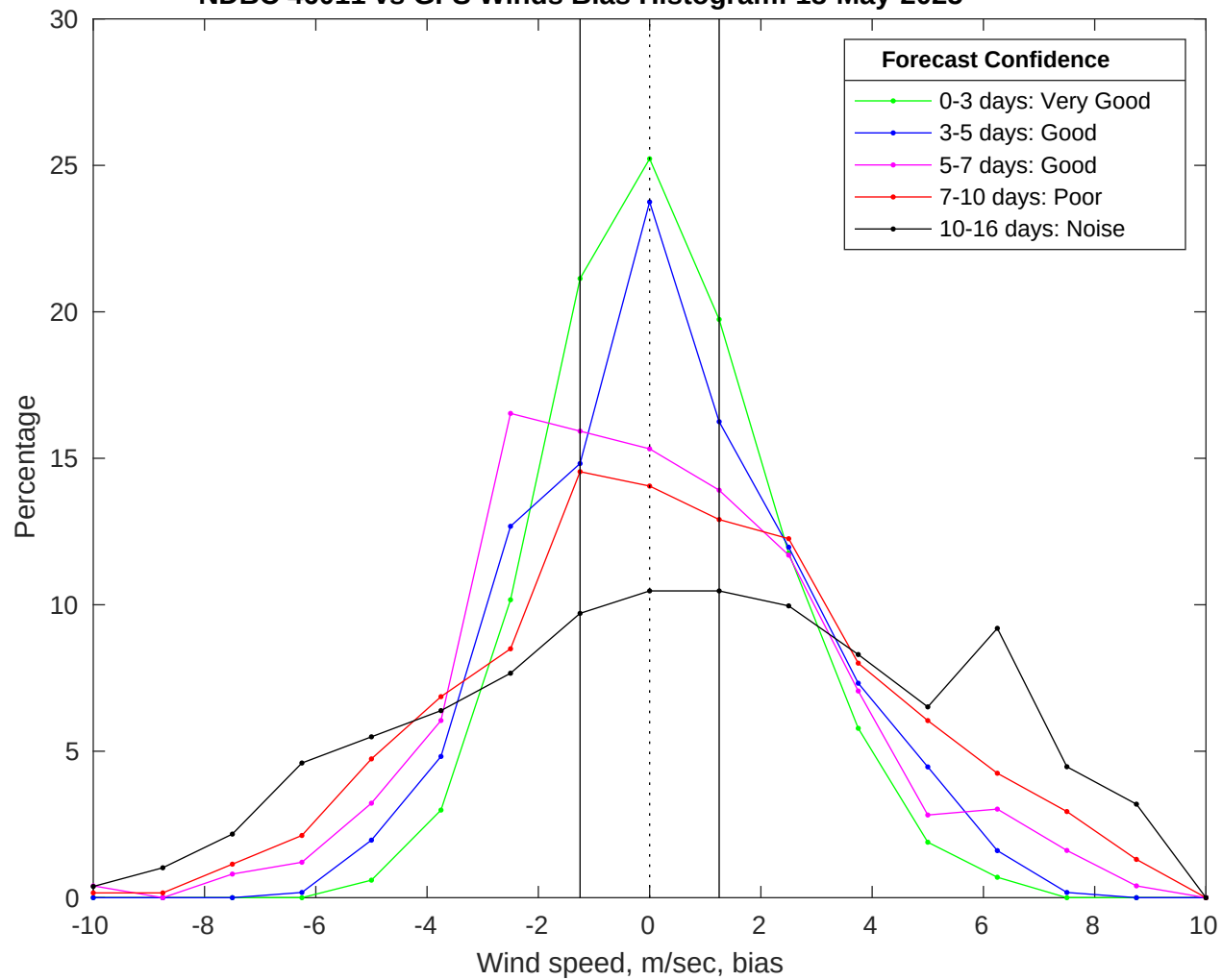
NDBC 46011 vs GFS Winds Bias Histogram: 18-May-2025
