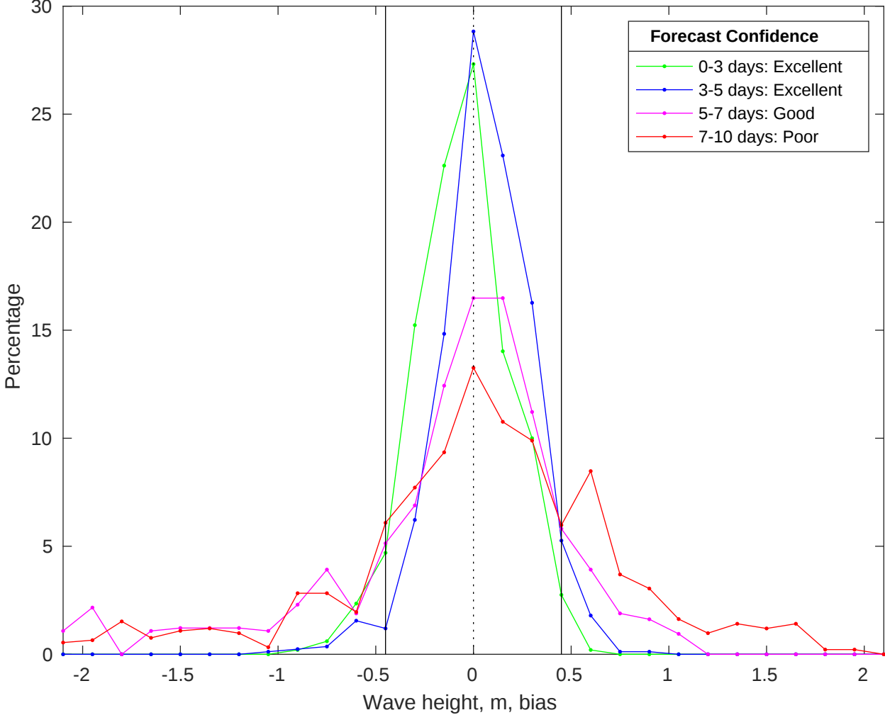
NDBC 46028 vs CMEMS Waves Bias Histogram: 18-May-2025
