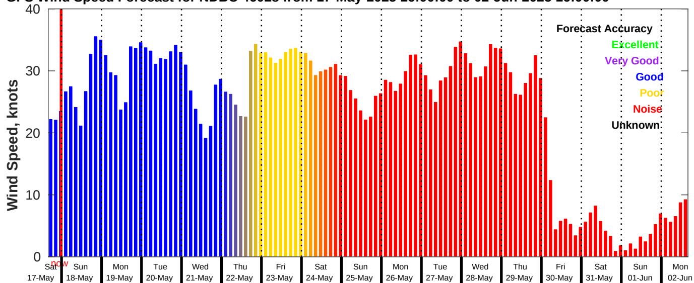
GFS Wind Speed Forecast for NDBC 46028 from 17-May-2025 16:00:00 to 02-Jun-2025 16:00:00
