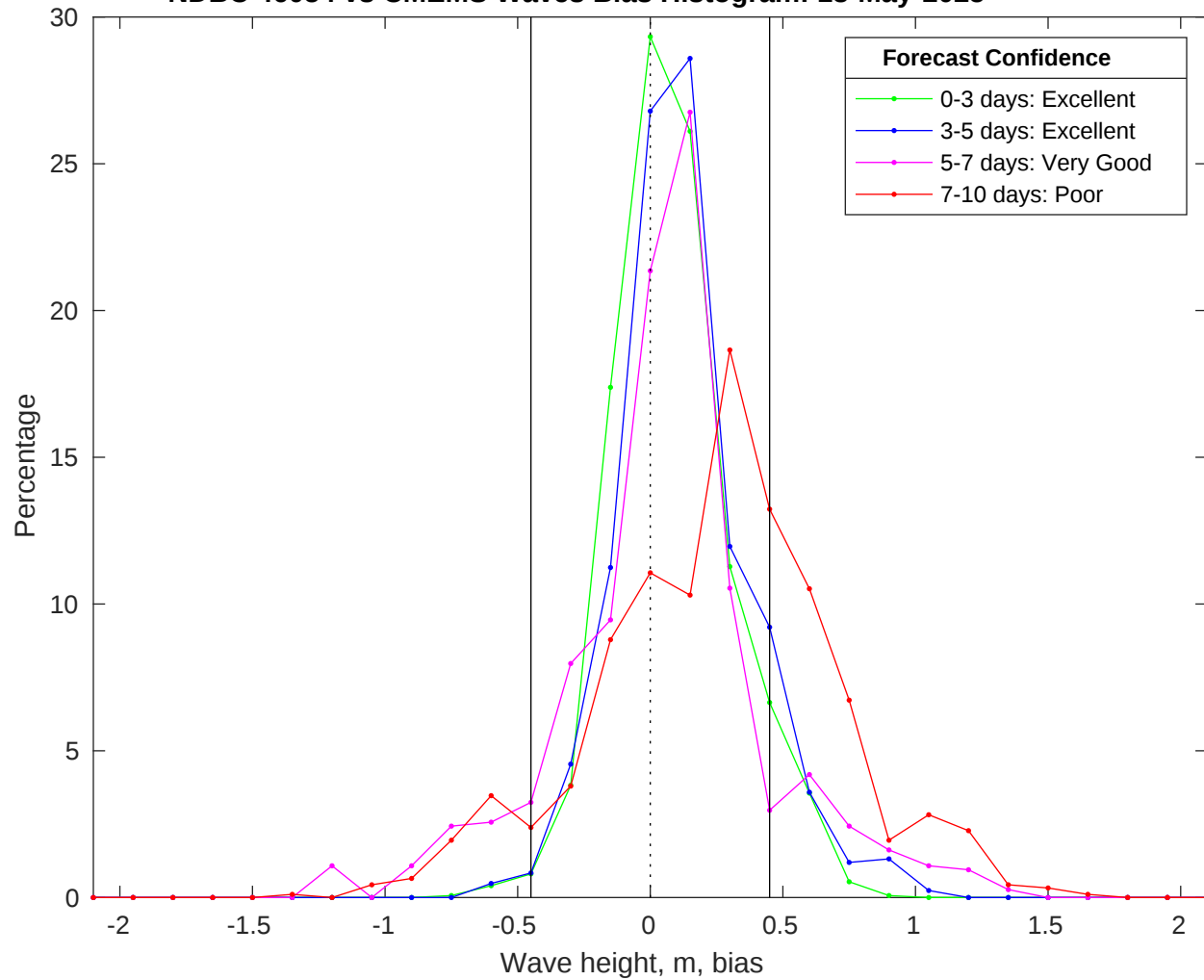
NDBC 46054 vs CMEMS Waves Bias Histogram: 18-May-2025
