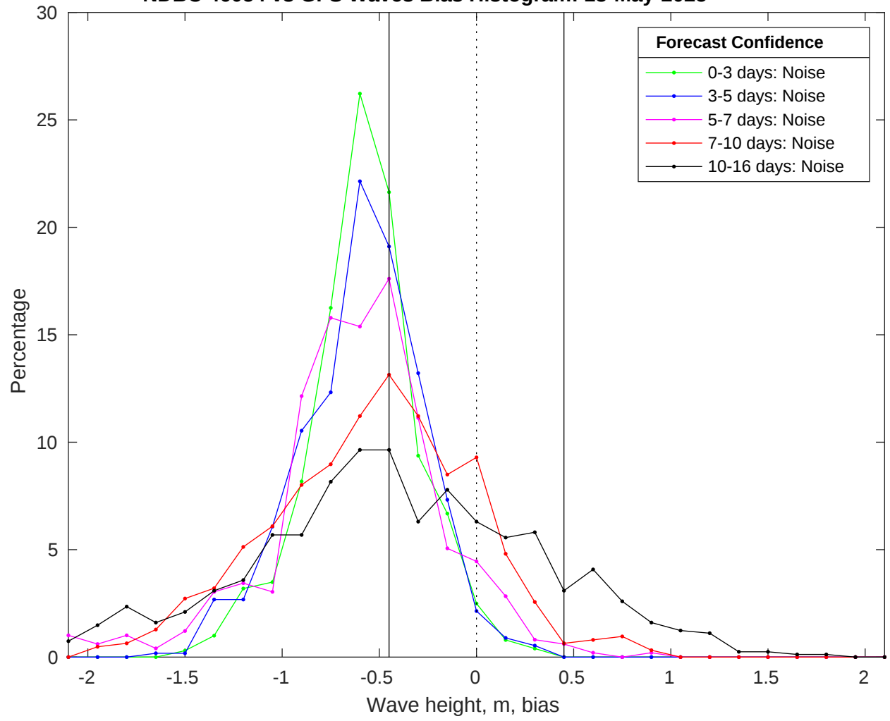
NDBC 46054 vs GFS Waves Bias Histogram: 18-May-2025
