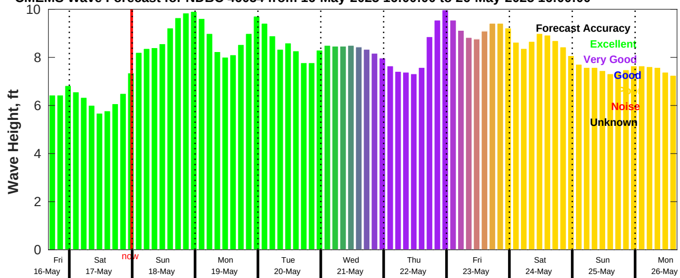
CMEMS Wave Forecast for NDBC 46054 from 16-May-2025 16:00:00 to 26-May-2025 16:00:00
