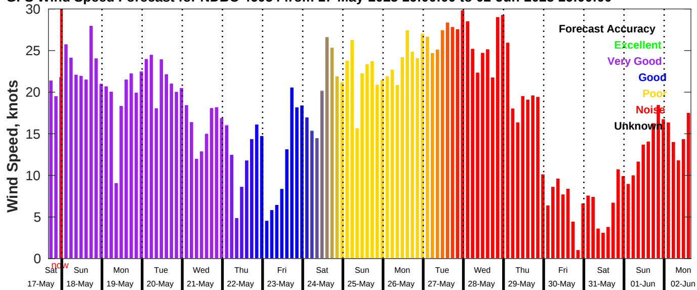
GFS Wind Speed Forecast for NDBC 46054 from 17-May-2025 16:00:00 to 02-Jun-2025 16:00:00
