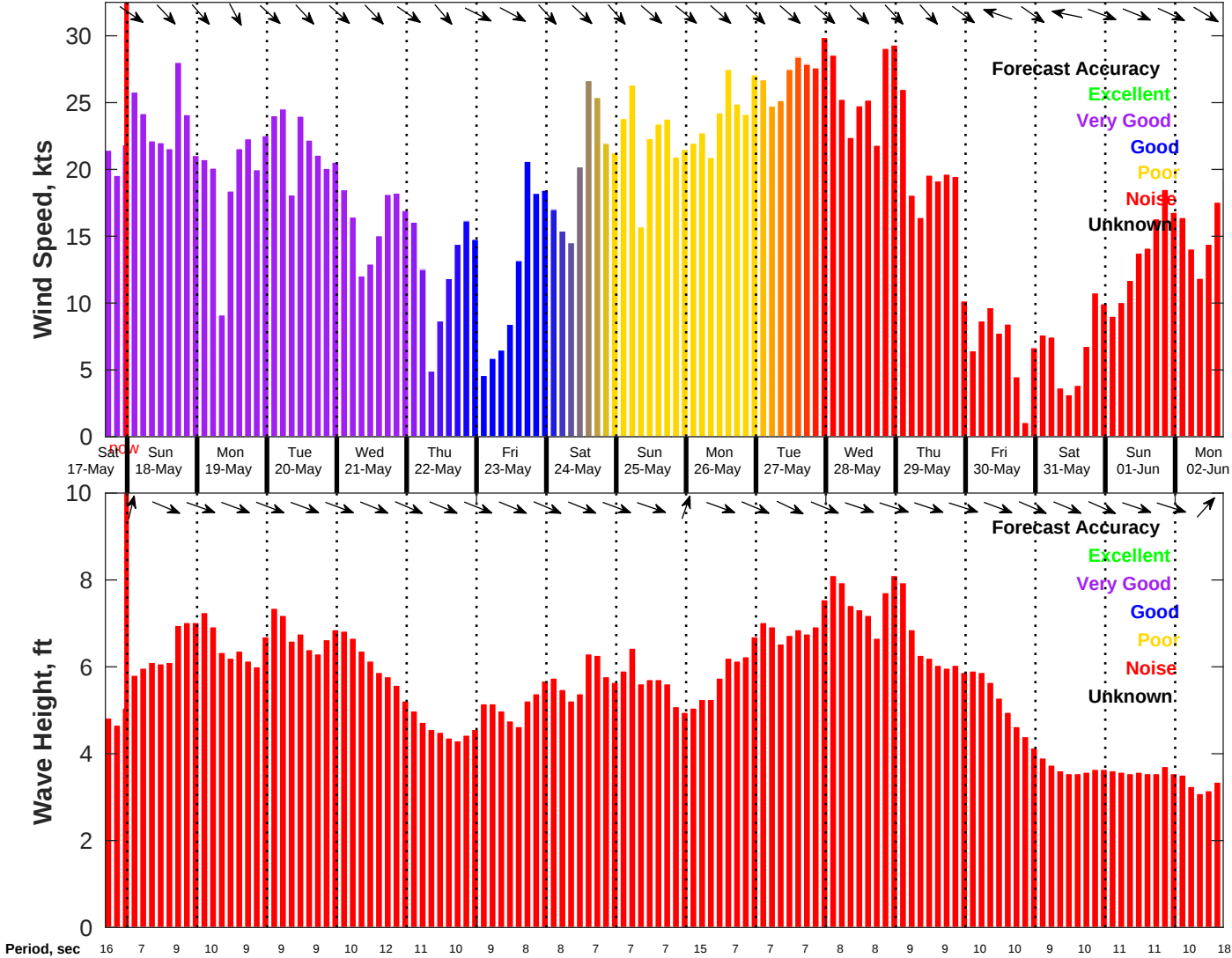
Wind & Wave Forecast for NDBC 46054 from 17-May-2025 16:00:00 to 02-Jun-2025 16:00:00
