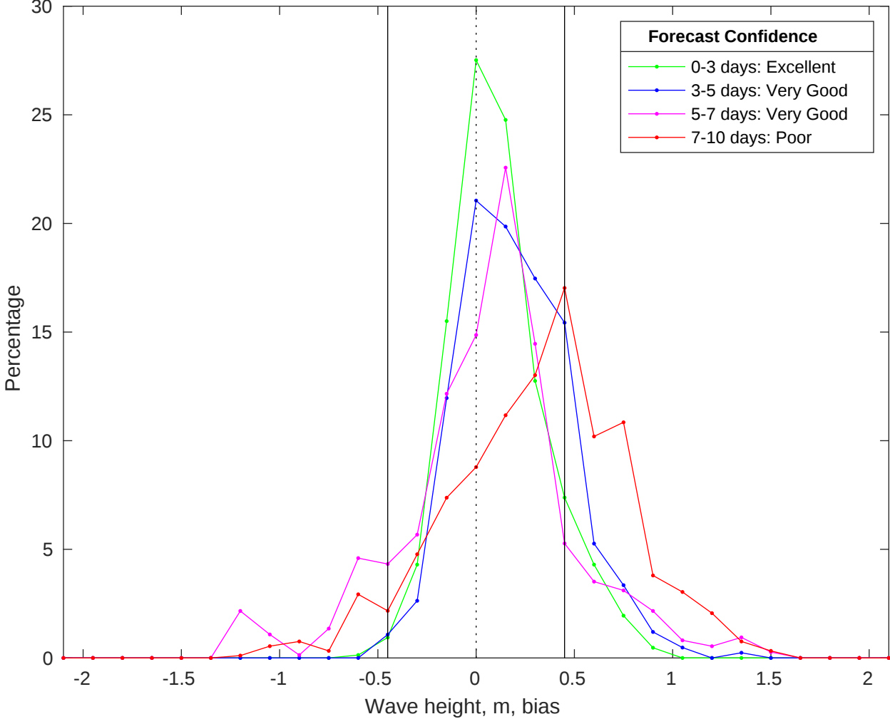
NDBC 46069 vs CMEMS Waves Bias Histogram: 18-May-2025
