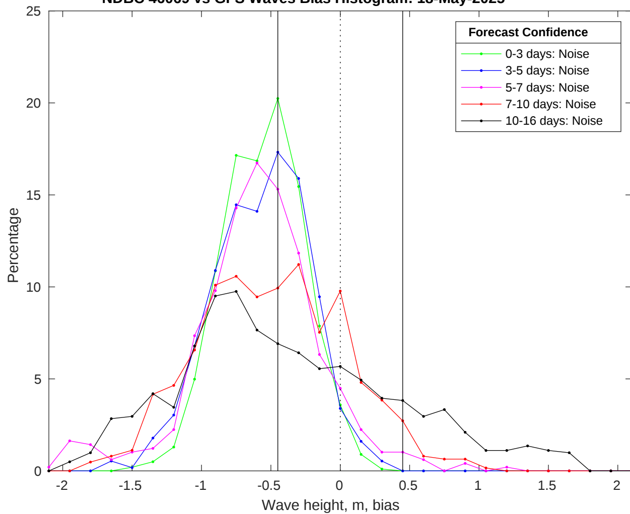
NDBC 46069 vs GFS Waves Bias Histogram: 18-May-2025
