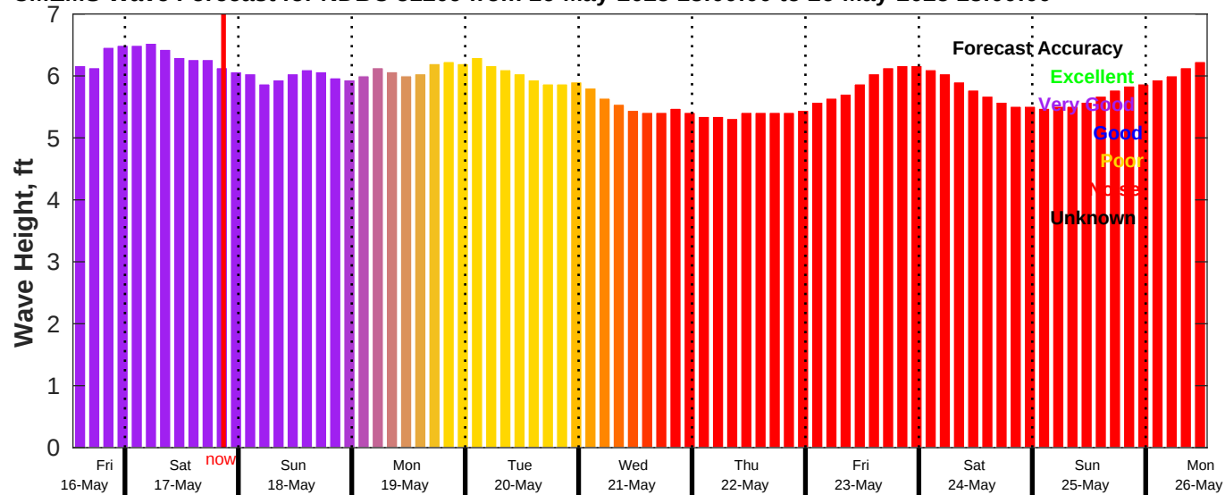
CMEMS Wave Forecast for NDBC 51209 from 16-May-2025 13:00:00 to 26-May-2025 13:00:00
