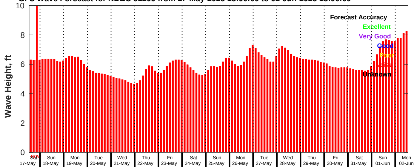
GFS Wave Forecast for NDBC 51209 from 17-May-2025 13:00:00 to 02-Jun-2025 13:00:00
