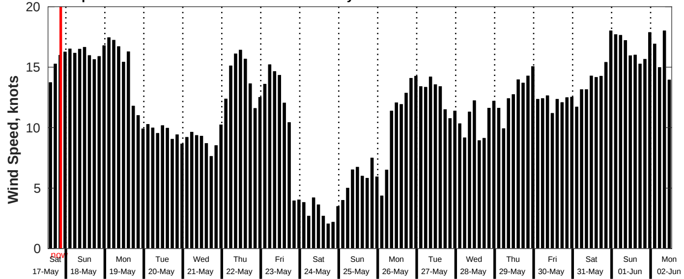
GFS Wind Speed Forecast for NDBC 51209 from 17-May-2025 13:00:00 to 02-Jun-2025 13:00:00
