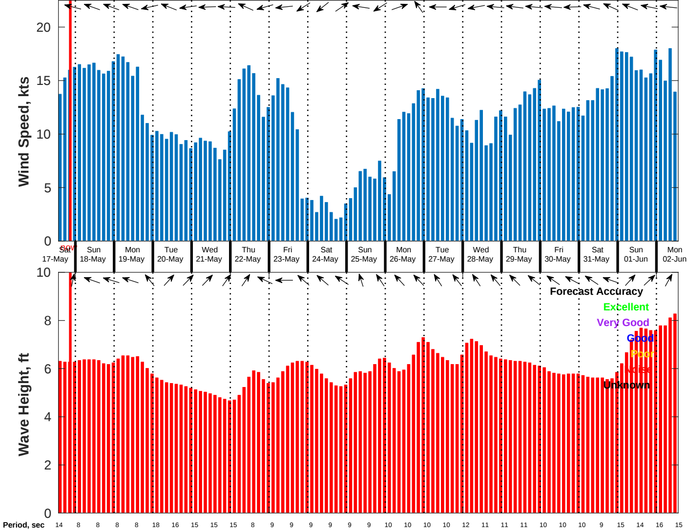
Wind & Wave Forecast for NDBC 51209 from 17-May-2025 13:00:00 to 02-Jun-2025 13:00:00
