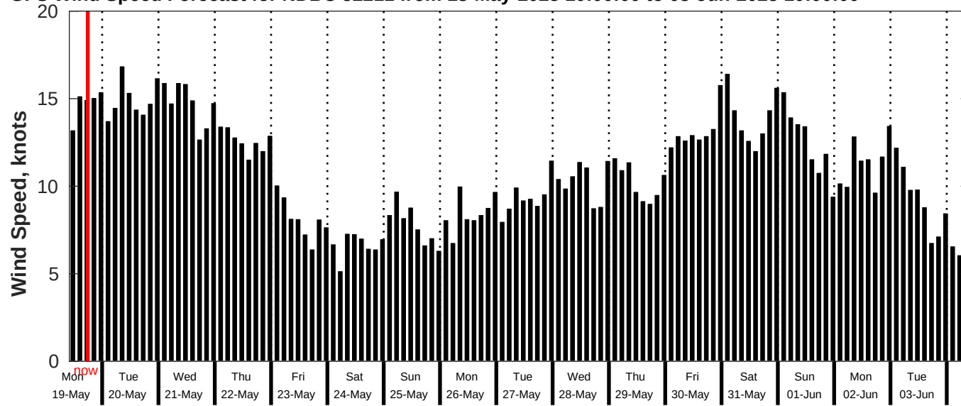
GFS Wind Speed Forecast for NDBC 52211 from 18-May-2025 10:00:00 to 03-Jun-2025 10:00:00
