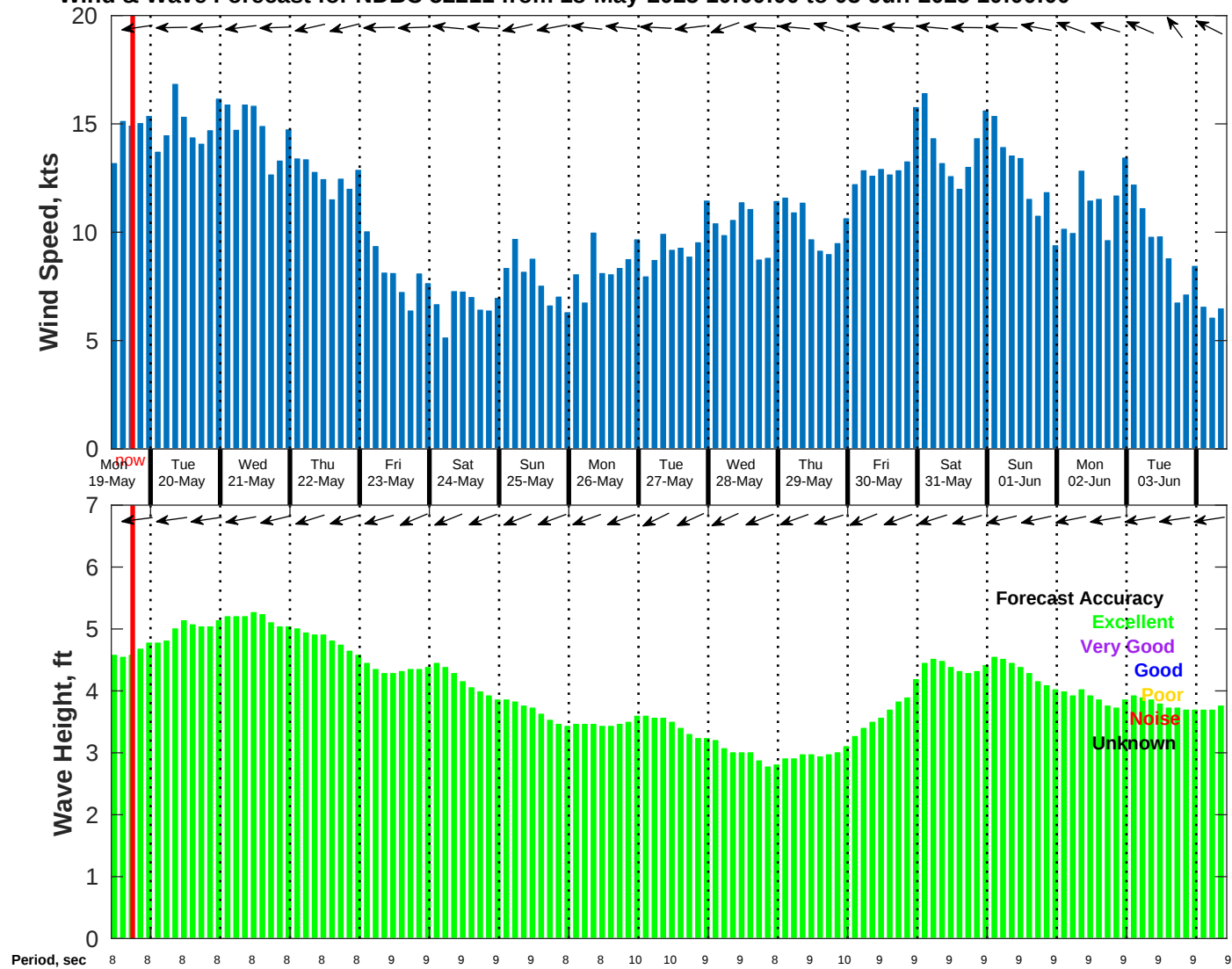
Wind & Wave Forecast for NDBC 52211 from 18-May-2025 10:00:00 to 03-Jun-2025 10:00:00
