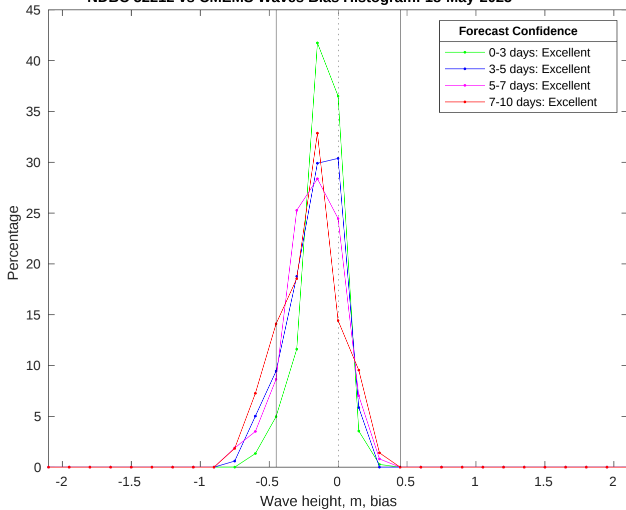
NDBC 52212 vs CMEMS Waves Bias Histogram: 18-May-2025
