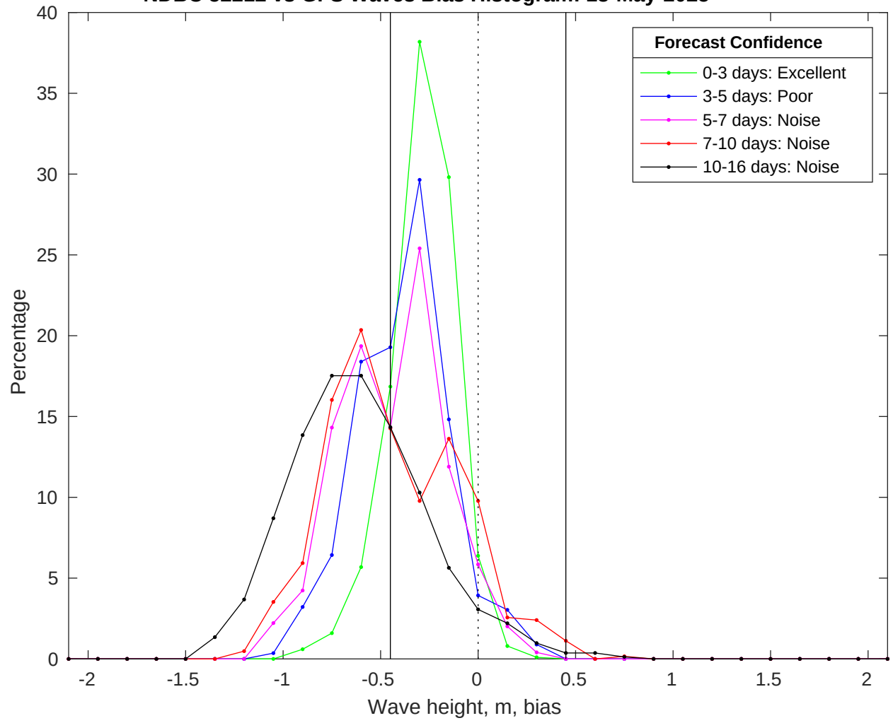
NDBC 52212 vs GFS Waves Bias Histogram: 18-May-2025
