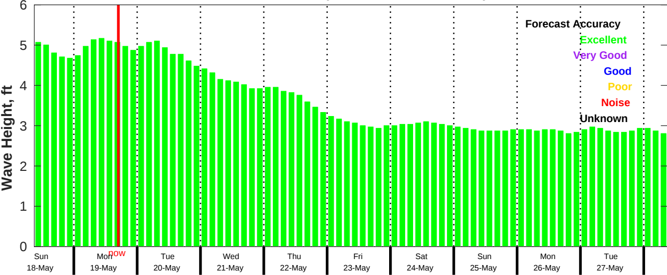
CMEMS Wave Forecast for NDBC 52212 from 17-May-2025 09:00:00 to 27-May-2025 09:00:00
