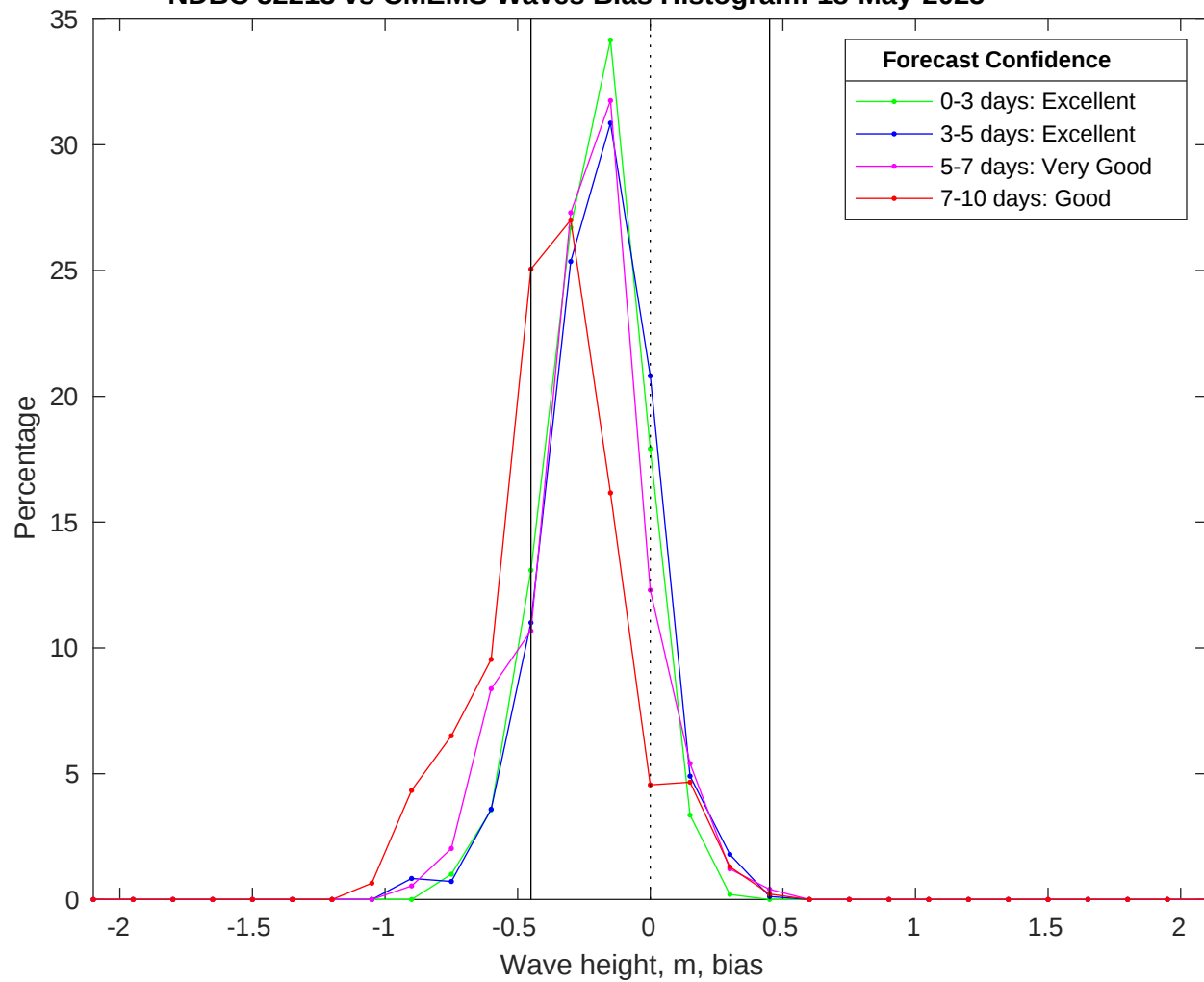
NDBC 52213 vs CMEMS Waves Bias Histogram: 18-May-2025
