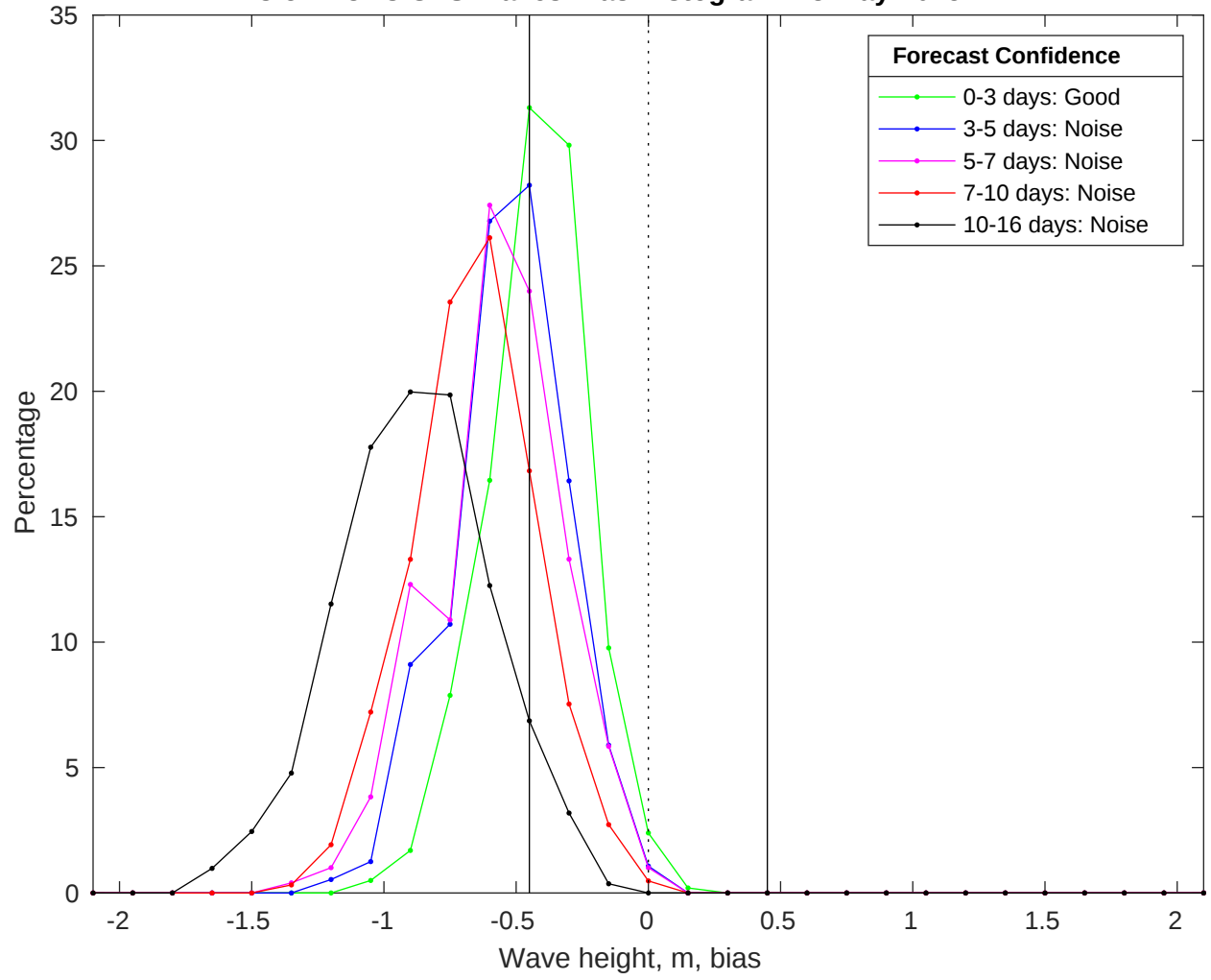
NDBC 52213 vs GFS Waves Bias Histogram: 18-May-2025
