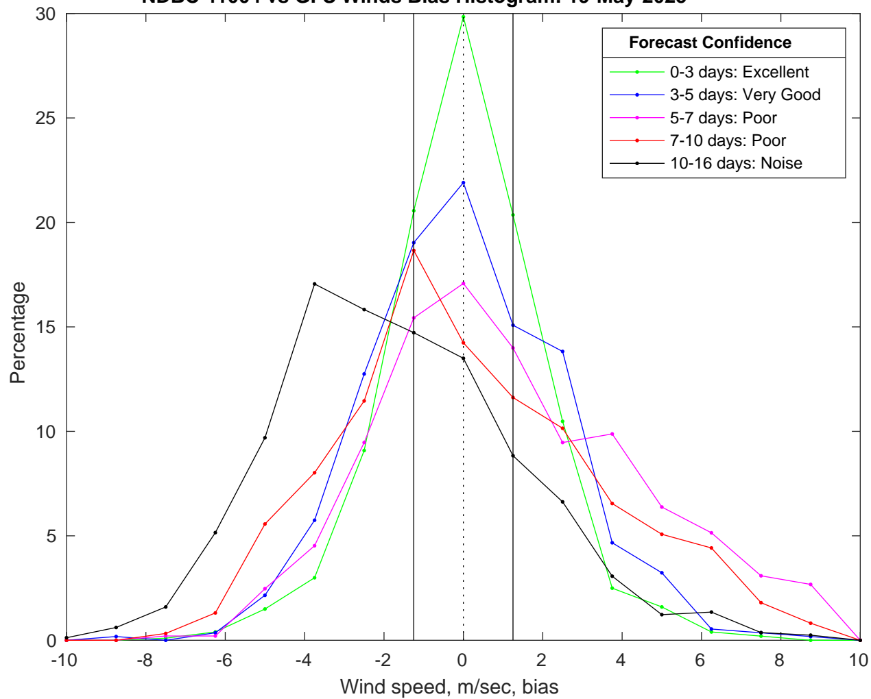
NDBC 41004 vs GFS Winds Bias Histogram: 19-May-2025
