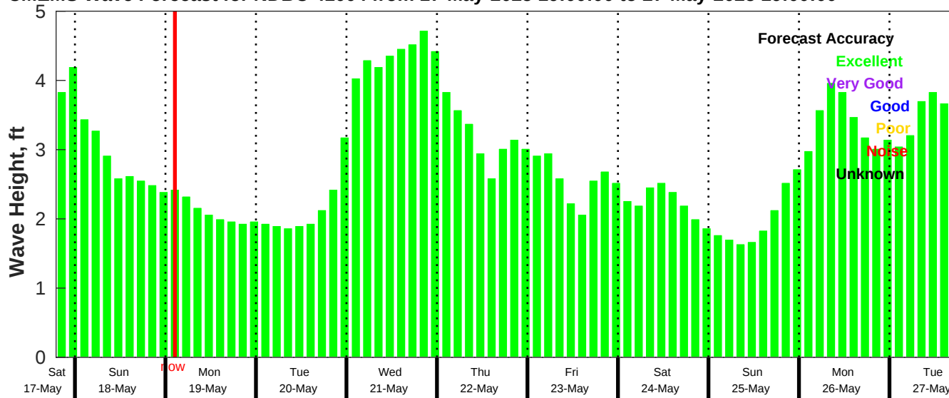
CMEMS Wave Forecast for NDBC 41004 from 17-May-2025 19:00:00 to 27-May-2025 19:00:00
