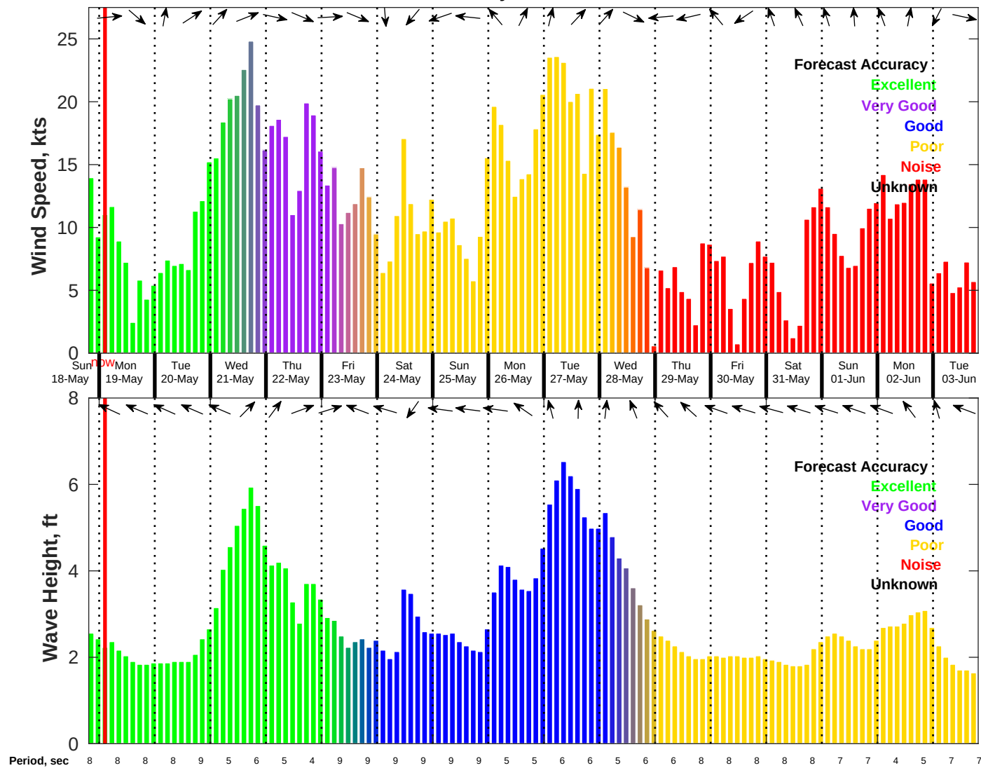
Wind & Wave Forecast for NDBC 41004 from 18-May-2025 19:00:00 to 03-Jun-2025 19:00:00
