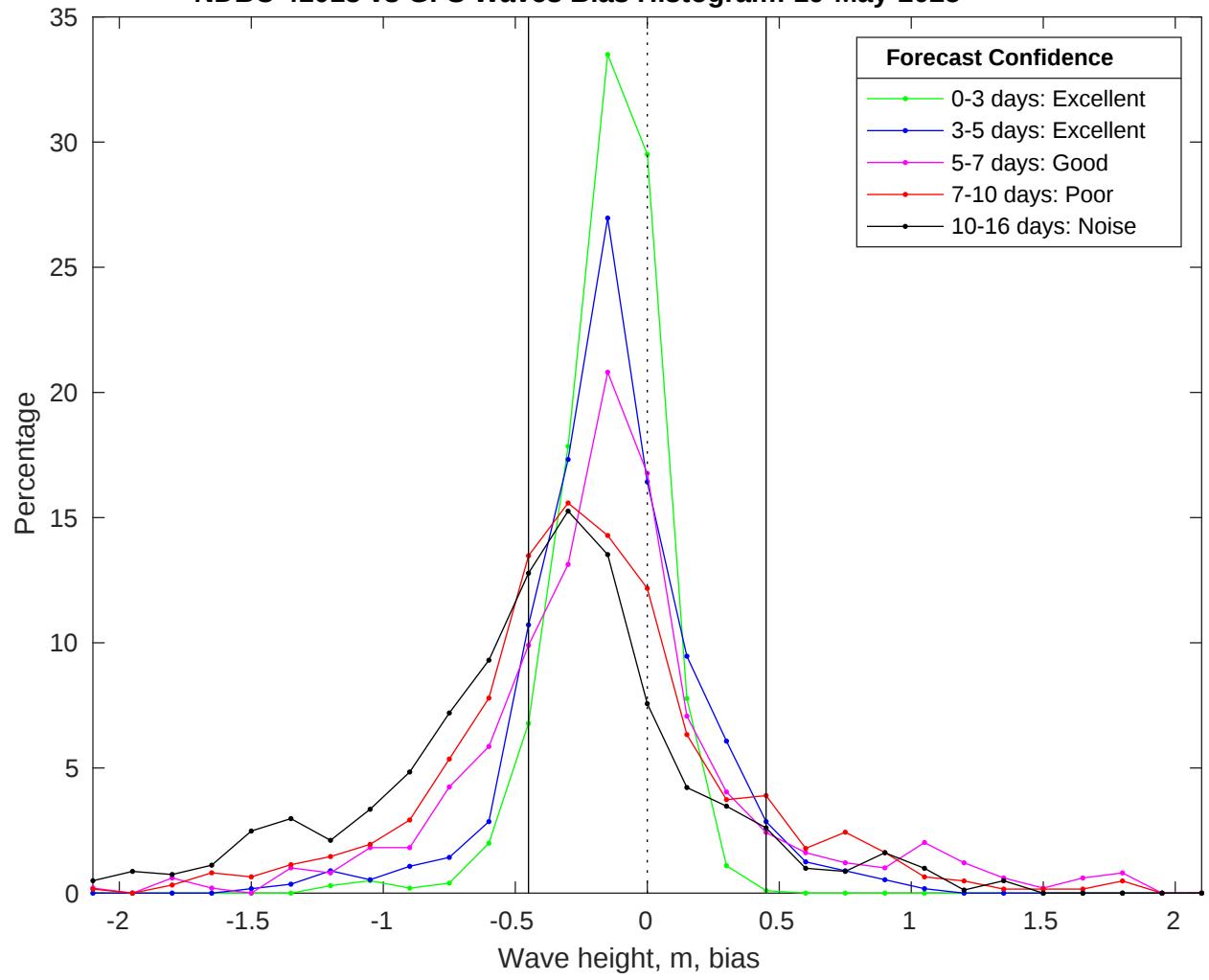
NDBC 41013 vs GFS Waves Bias Histogram: 19-May-2025
