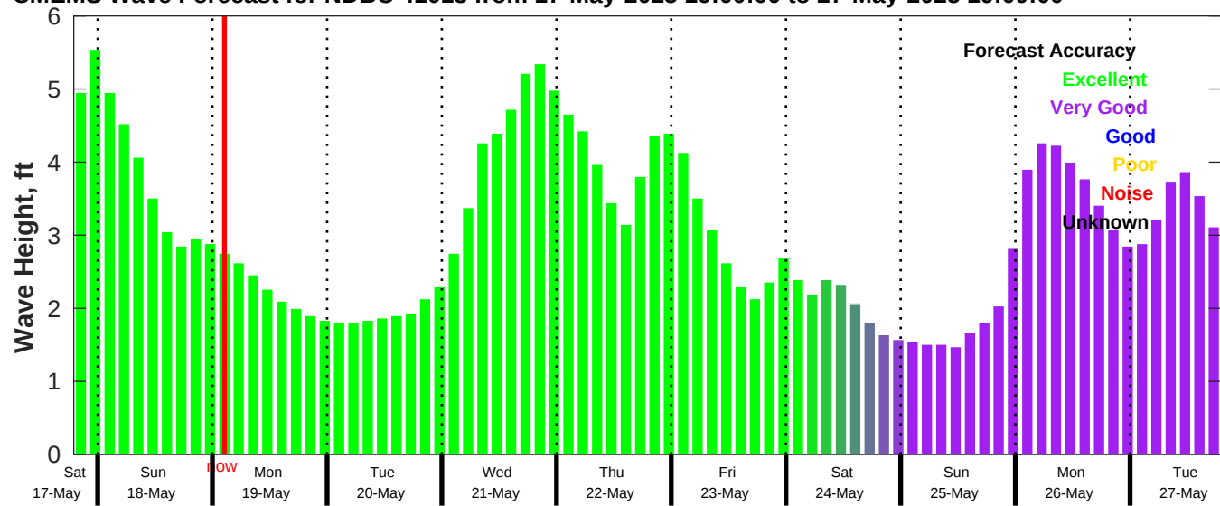
CMEMS Wave Forecast for NDBC 41013 from 17-May-2025 19:00:00 to 27-May-2025 19:00:00
