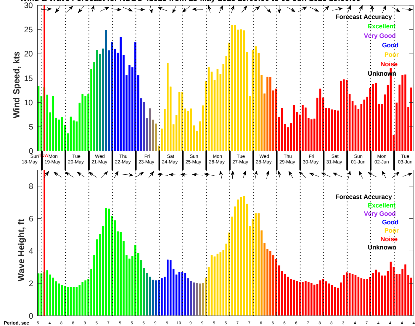
Wind & Wave Forecast for NDBC 41013 from 18-May-2025 19:00:00 to 03-Jun-2025 19:00:00
