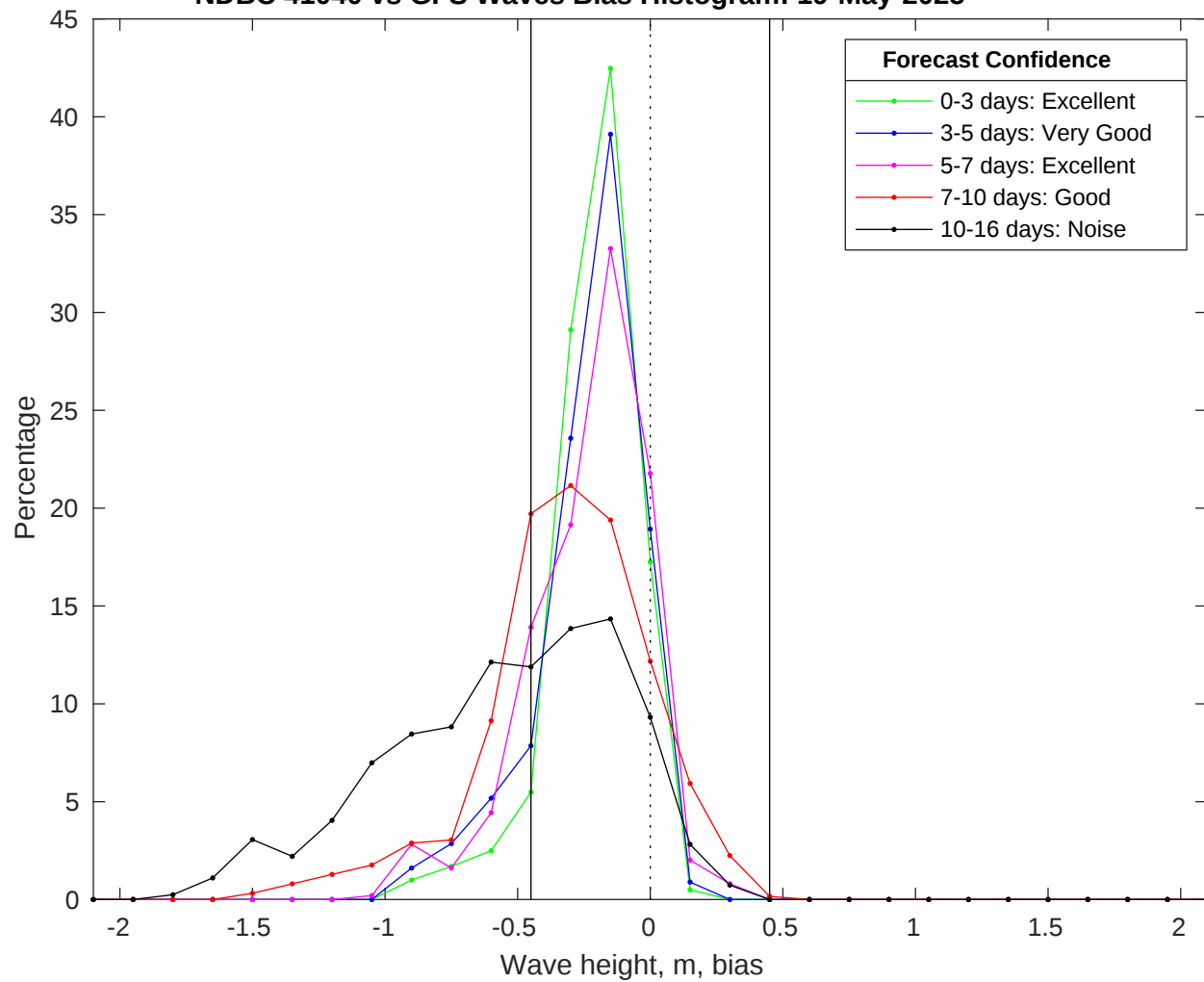
NDBC 41040 vs GFS Waves Bias Histogram: 19-May-2025
