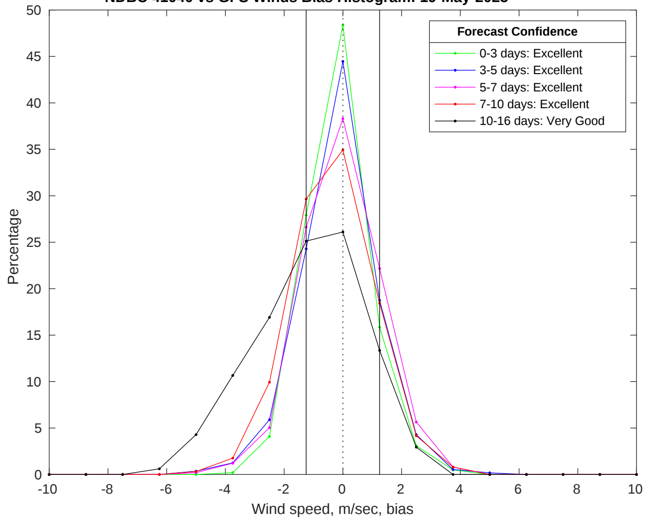
NDBC 41040 vs GFS Winds Bias Histogram: 19-May-2025
