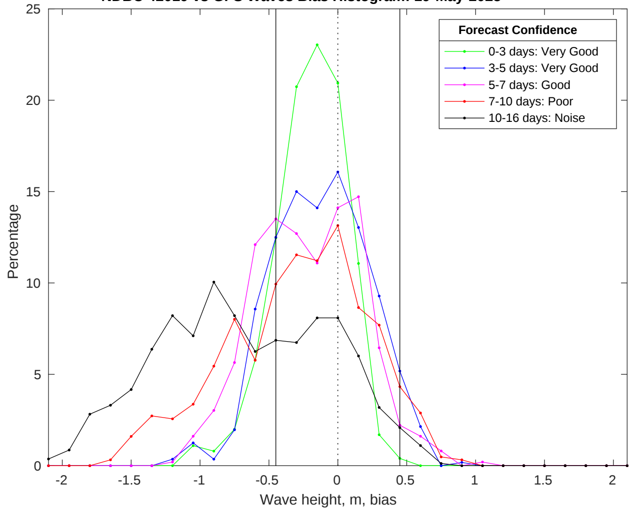
NDBC 42019 vs GFS Waves Bias Histogram: 19-May-2025
