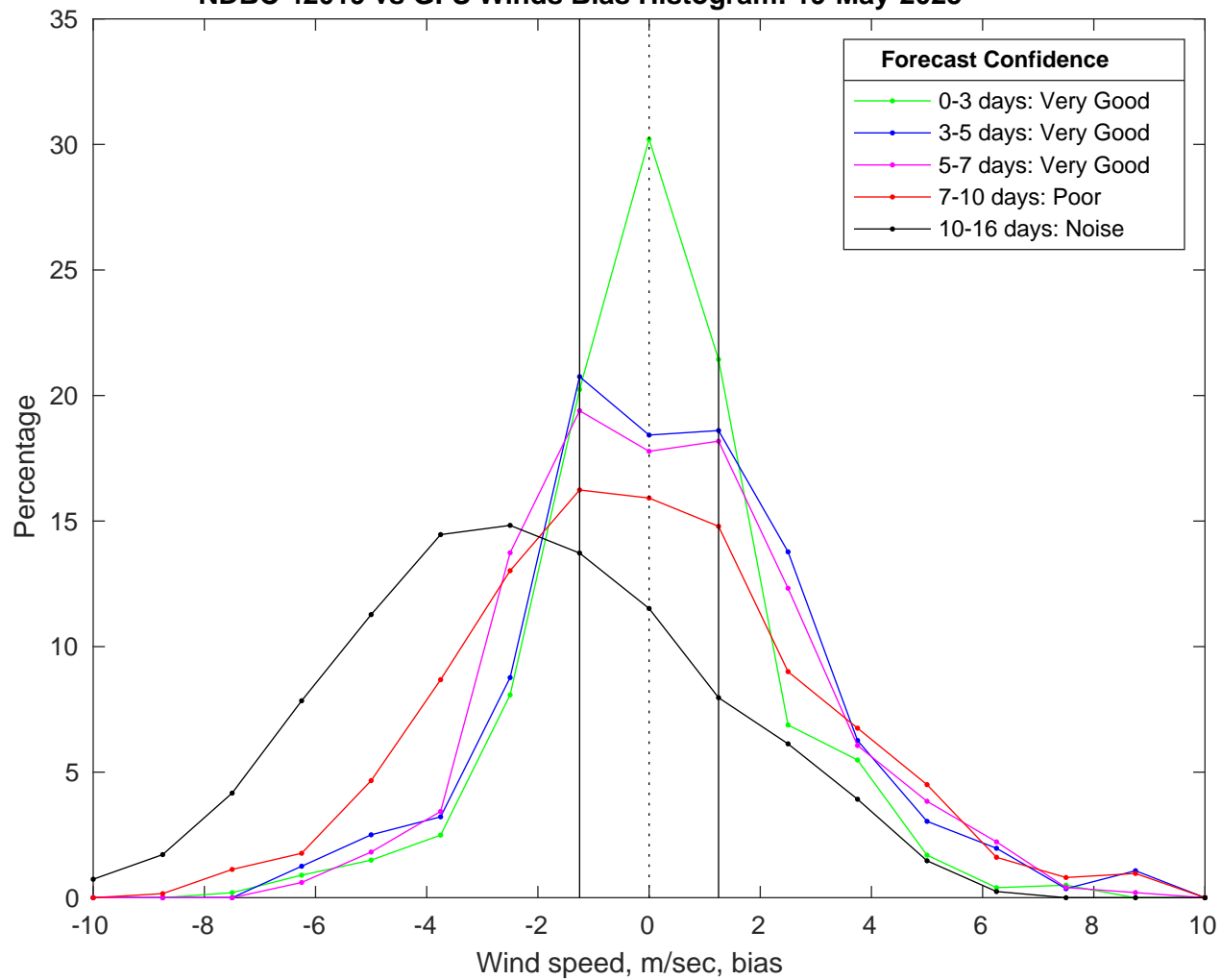
NDBC 42019 vs GFS Winds Bias Histogram: 19-May-2025
