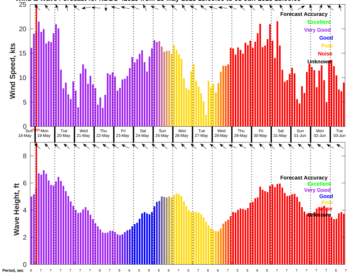
Wind & Wave Forecast for NDBC 42019 from 18-May-2025 18:00:00 to 03-Jun-2025 18:00:00
